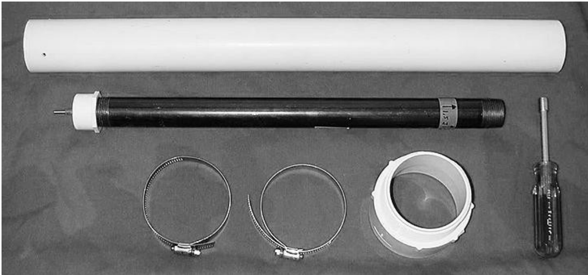
Figure 5 - Parts needed for SCA Standard Drop Tester for fencing armor.
